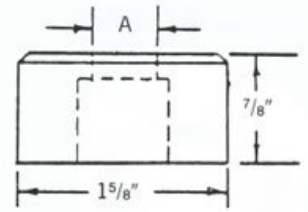
* Fig. No. 125 "A" to 1 1/8"
