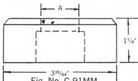
Fig. No. C-91MM "A" 1 3/32" to 2 5/16"
