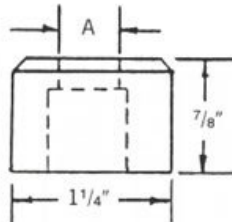
Fig. No. 43 "A" 5/32" to 1"
