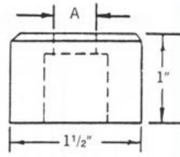
Fig. No. 46 "A" 5/32" to 1 3/16"
